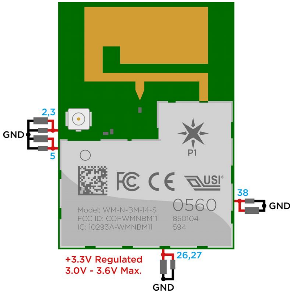
Fig. 1 Recommended power connections with decoupling capacitors. RF
